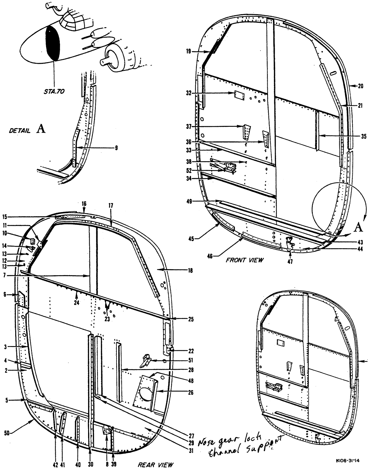
Figure 23 FUSELAGE STATION 70 FRAME ASSEMBLY
