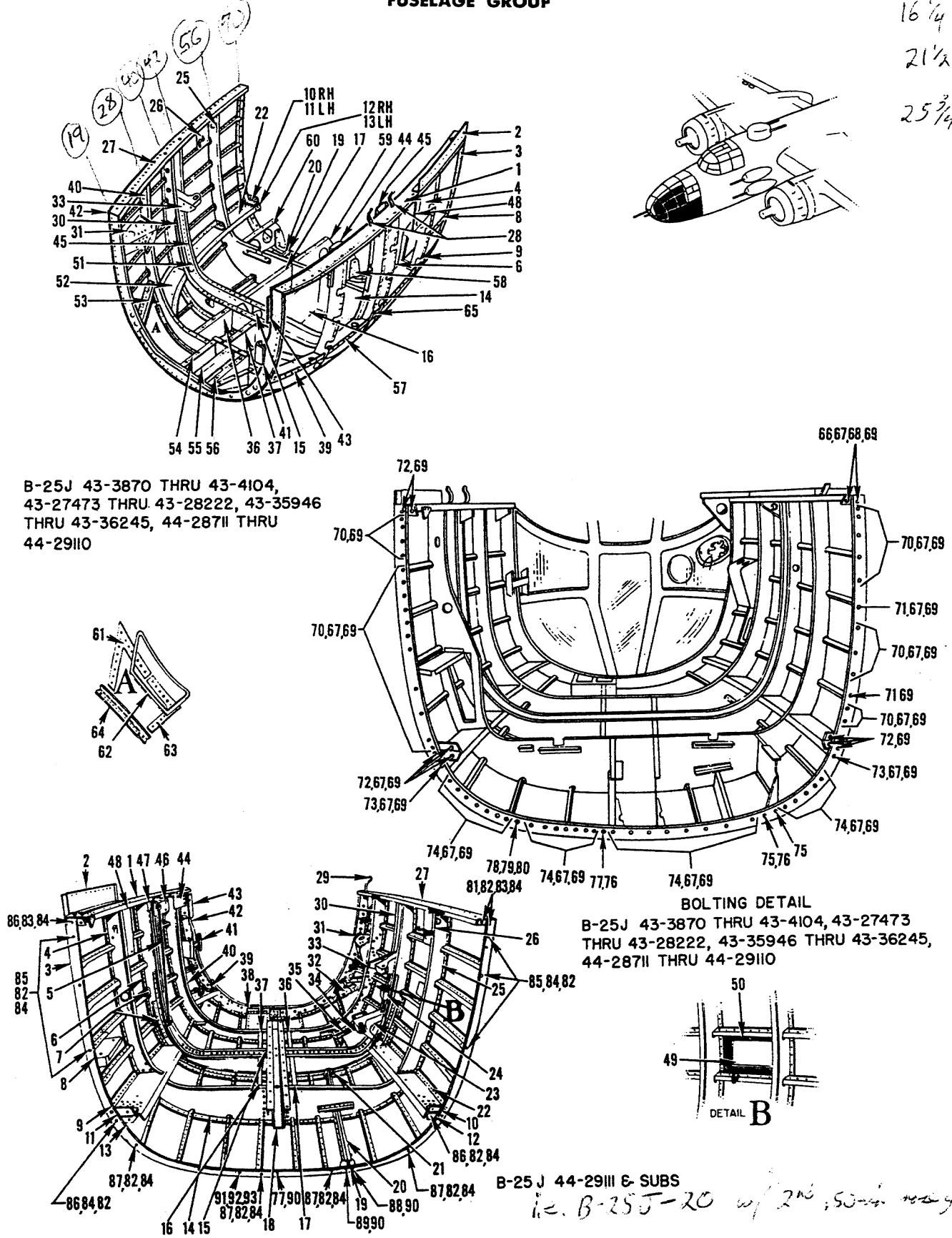
Figure 22 BOMBARDIER'S BOTTOM FUSELAGE STATION 19 TO 70 FRAME ASSEMBLY (B-25J)
