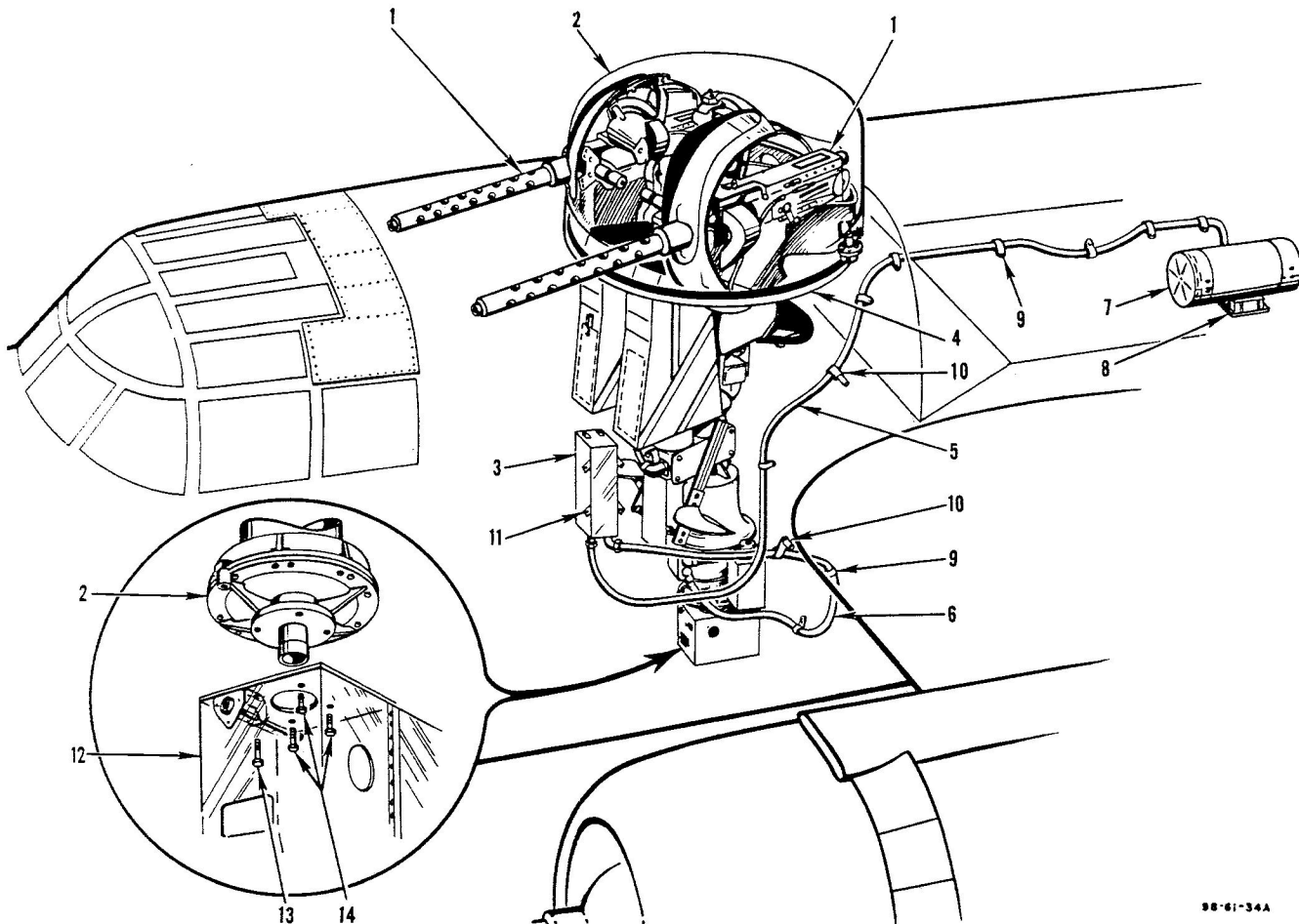
Figure 289 UPPER GUN TURRET INSTALLATION
